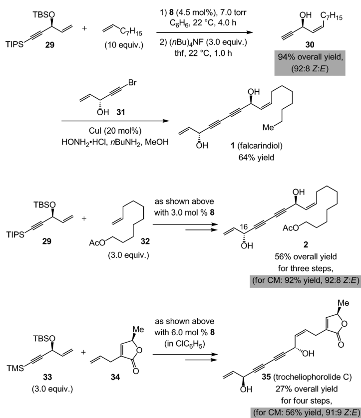
Scheme 5. Application of Z-selective CM of allylic ethers to the preparation of faltarindiol ( 1 ) and derivatives 2 and 35 (proposed structure), which possess anticancer, antifungal, and immunosuppressive activity. TIPS = triisopropylsilyl, TMS = trimethylsilyl.
