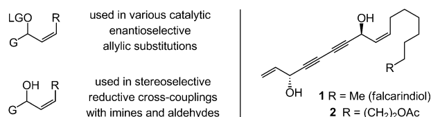
Scheme 1. Z -Allylic alcohols and their derivatives serve as substrates in stereoselective transformations (left), and reside in biologically active molecules (right). G = functional group, LG = leaving group.
